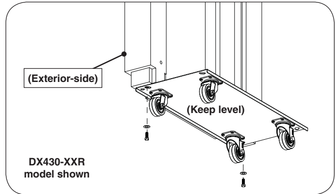
Fig. 2-1 Install left wheel assembly to bottom of left side wall
