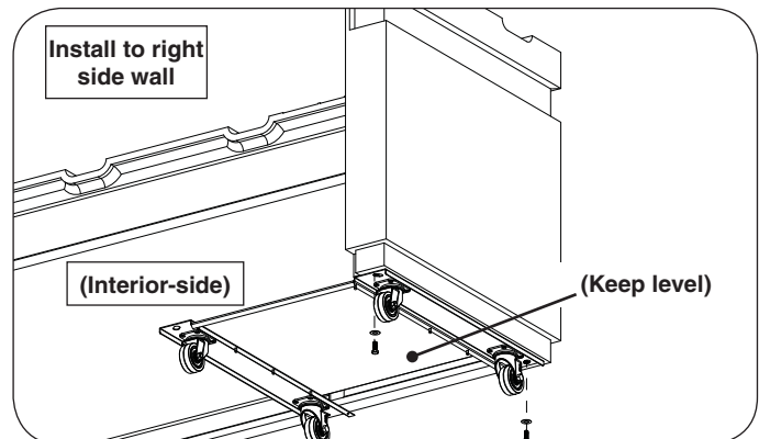
Fig. 2-3 Install right wheel assembly to bottom of right side wall
