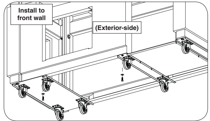
Fig. 3-1 Install wheel assemblies to bottom of front wall
