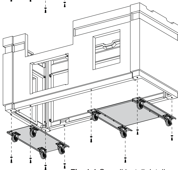
Fig. 1-1 Overall install detail
