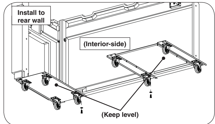
Fig. 2-2 Install wheel assemblies to bottom of rear wall
